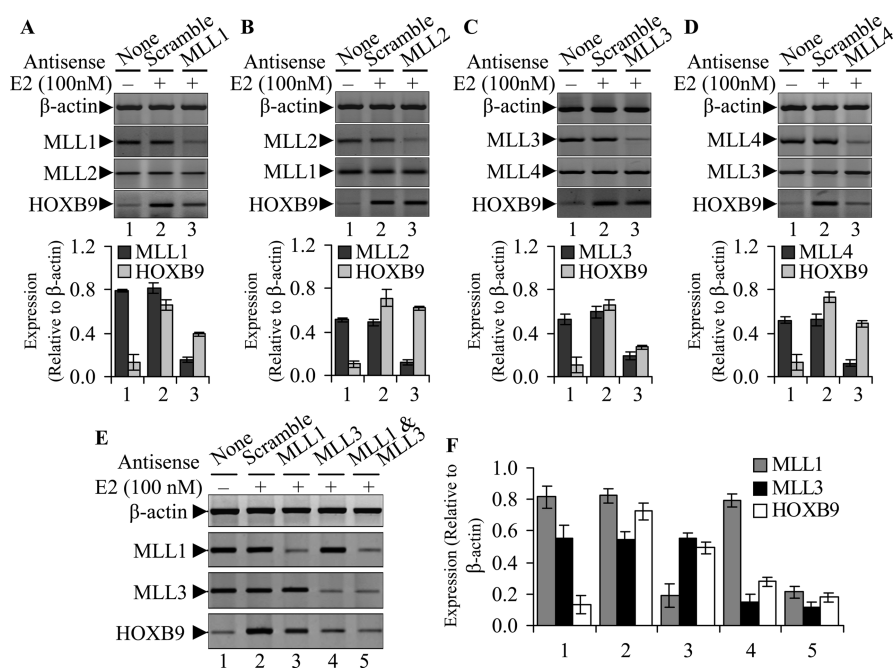
Figure 5. Effect of knockdown of MLL1, MLL2, MLL3, and MLL4 on E2-induced expression of HOXB9. JAR cells were transfected with 5 \mu g of MLL1, MLL2, MLL3, and MLL4 specific antisense oligonucleotides separately. Control cells were treated with a scramble antisense with no homology with MLLs. The antisense-treated cells were incubated for 48 h followed by treatment with 100 nM E2 for 6 h. RNA was isolated from treated and control cells and subjected to reverse transcriptase-PCR by using primers specific to HOXB9 along with MLL1, MLL2, MLL3, and MLL4. \beta -Actin was used as control. The PCR products were analyzed by agarose gel. Quantification of transcript accumulation was done by using real-time PCR (shown in respective bottom panel). (A) Effect of MLL1 knockdown. (Top) Lane 1: control cells (no E2 treatment); lane 2: cells that were initially transfected with scramble antisense followed by exposure to E2; lanes 3: cells were initially transfected with MLL1 antisense and then treated with E2. Real-time PCR analysis of the expression profiles of MLL1 and HOXB9 (relative to \beta -actin, average of three replicate experiments, n = 3 ) were quantified and plotted in the bottom panel. MLL2 was used as control to determine target specificity of MLL1 antisense. (B–D) These figures show the effects of knockdown of MLL2 (MLL1 as control), MLL3 (MLL4 as control), and MLL4 (MLL3 as control), respectively, in a similar manner as shown for MLL1 in panel A. (E, F) Effect of combined knockdown of MLL1 and MLL3 in E2-induced HOXB9 expression. The knockdown experiments were performed in the same way as shown in panels A–D. For combined knockdown (lane 5), MLL1 and MLL3 antisenses were mixed together in equimolar amounts and then transfected. Real-time PCR analyses of the expression profiles of MLL1, MLL3, and HOXB9 are plotted in panel F.
