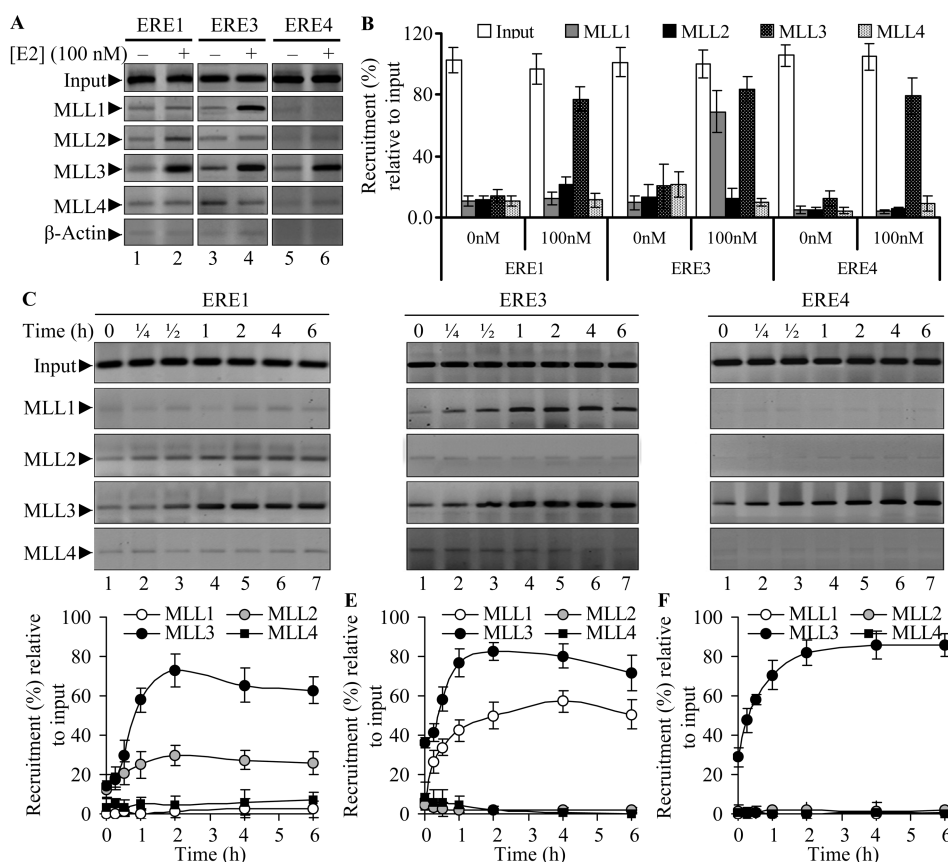
Figure 6. E2-dependent recruitment of MLLs (MLL1–4) in ERE1, ERE3, and ERE4 of HOXB9 promoter. (A, B) JAR cells were treated with 100 nM E2 for 6 h and subjected to ChIP assay using antibodies specific to MLL1, MLL2, MLL3, and MLL4. \beta -actin antibody was used as control IgG. The immunoprecipitated DNA fragments were PCR-amplified using primers specific to ERE1, ERE3, and ERE4 of HOXB9 promoter. Lanes 1, 3, and 5 are no-E2 controls. Lanes 2, 4, and 6 are E2-treated samples. ChIP DNA fragments were analyzed by real-time PCR and shown in panel B. Each experiment was repeated at least thrice. Bars indicate standard errors. (C) Dynamics of recruitment of MLL1, MLL2, MLL3, and MLL4 onto HOXB9 promoter: Cells were treated with 100 nM E2 for varying time periods and then subjected to ChIP assay using antibodies specific to MLL1, MLL2, MLL3, and MLL4. Immunoprecipitated DNA fragments were PCR-amplified using primers specific to ERE1, ERE3, and ERE4 of HOXB9 promoter. Lane 1: control cells (no E2 control). Quantifications of recruitment level (% relative to input) are plotted in respective bottom panels. Bars indicate standard errors.
