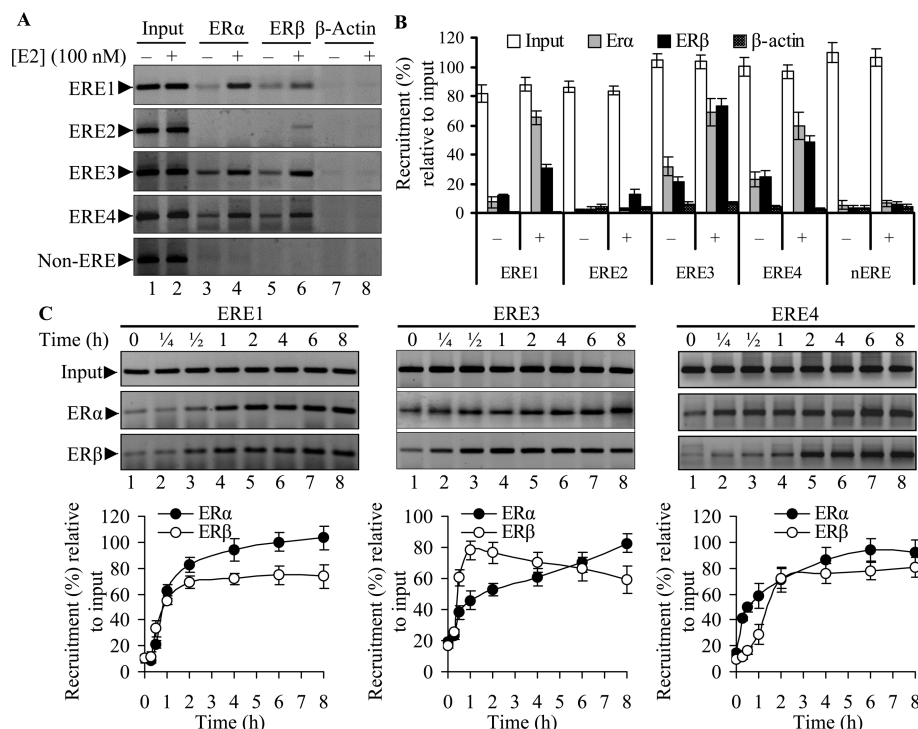
Figure 4. E2-dependent recruitment of ER \alpha and ER \beta in the ERE regions of HOXB9 promoter. (A, B) JAR cells were treated with 100 nM E2 for 6 h and subjected to ChIP assay using antibodies specific to ER \alpha and ER \beta . \beta -Actin antibody was used as control IgG. The immunoprecipitated DNA fragments were PCR-amplified using primers specific to ERE1–4 of HOXB9 promoter. Primers specific to a promoter sequence containing no ERE (non-ERE) were used as control. Lanes 1, 3, 5, and 7 are no-E2 controls. Lanes 2, 4, 6, and 8 are E2-treated samples. ChIP DNA fragments were analyzed by real-time PCR and shown in panel B. Each experiment was repeated at least thrice. Bars indicate standard errors. (C) Dynamics of recruitments of ER \alpha and ER \beta onto ERE1, ERE3, and ERE4 of HOXB9 promoter: Cells were treated with 100 nM E2 for varying time periods and then subjected to ChIP assay using antibodies specific to ER \alpha and ER \beta . Immunoprecipitated DNA fragments were PCR-amplified using primers specific to ERE1, ERE3, and ERE4 of HOXB9 promoter. Lane 1: control cells (no E2 treatment control). Quantification of recruitment level (% relative to input) is plotted in respective bottom panels. Bars indicate standard errors.
