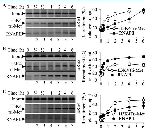
Figure 7. E2-dependent enrichment of H3K4-trimethylation level and recruitment of RNA polymerase II (RNAP II) in the ERE1, ERE3, and ERE4 of HOXB9 promoter. (A–C) JAR cells were treated with 100 nM E2 for varying time periods (0–6 h) and then subjected to ChIP assay using antibodies specific to H3K4-trimethylation and RNAPII. Immunoprecipitated DNA fragments were PCR amplified using primers specific to ERE1, ERE3, and ERE4 of HOXB9 promoter, respectively. Lane 1: control cells (no E2 control). Lanes 2–7 are E2-treated samples. Quantifications of recruitment level (% relative to input) are plotted in respective right panels. Bars indicate standard errors.
