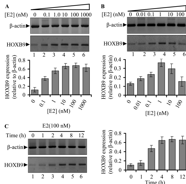
Figure 1. Effect of E2 on HOXB9 expression. (A) JAR cells (grown in phenol-red free media) were treated with varying concentrations of E2. RNA was isolated, reverse transcribed, and subjected to regular PCR (top panel) and real-time PCR (bottom panel) using primers specific to HOXB9. β-Actin was used as a loading control. Each experiment was repeated at least thrice. Bars indicate standard errors ( p < 0.05 ). (B) Effect of E2 on HOXB9 expression in MCF7 cells was analyzed in a similar way as described for JAR cells in (A). Top panel shows the agarose gel analysis of the PCR products, and bottom panel shows the real-time PCR data. (C) JAR cells were treated with 100 nM E2 for varying time periods (0–12 h), and RNA was reverse transcribed and analyzed by regular PCR (left panel) and real-time PCR (right panel) using HOXB9 and β-actin primers. Each experiment was repeated at least thrice ( n = 3 ).
