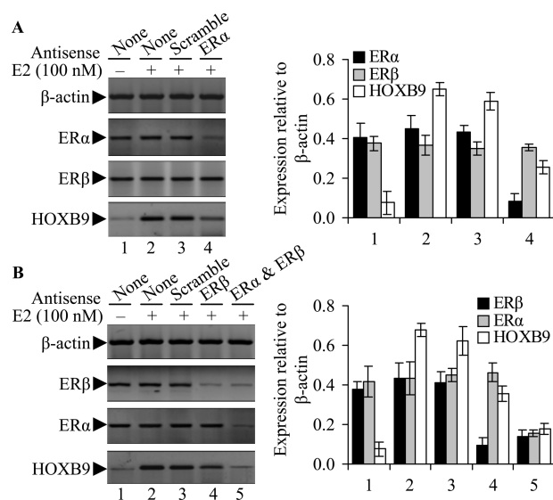
Figure 3. Roles of ER \alpha and ER \beta in E2-induced expression of HOXB9. (A) Effect of ER \alpha knockdown: JAR cells were transfected with ER \alpha and a scramble antisense (9 \mu g each) for 48 h. Antisense-transfected cells were treated with E2 (100 nM for 6 h). RNA was isolated and subjected to reverse transcriptase-PCR analysis by using primers specific to ER \alpha and HOXB9. PCR with ER \beta was done to confirm specificity of ER \alpha antisense and \beta -actin was used quantitative control. PCR products were analyzed in agarose gel. Lane 1: control cells (no E2 control); lane 2: cells were treated with 100 nM E2; lane 3: cells were initially transfected with 9 \mu g of scramble antisense followed by exposure to E2; lane 4: cells were initially transfected with 9 \mu g of ER \alpha antisense and then treated with E2. Real-time PCR analysis of ER \alpha , ER \beta , and HOXB9 relative to \beta -actin is plotted. Each experiment was repeated at least thrice ( n = 3 ). Bars indicate standard errors. (B) Effect of ER \beta knockdown or a combined knockdown of ER \alpha and ER \beta on E2-induced HOXB9 expression. Experiments and analysis were performed in the same way as shown in panel A.
