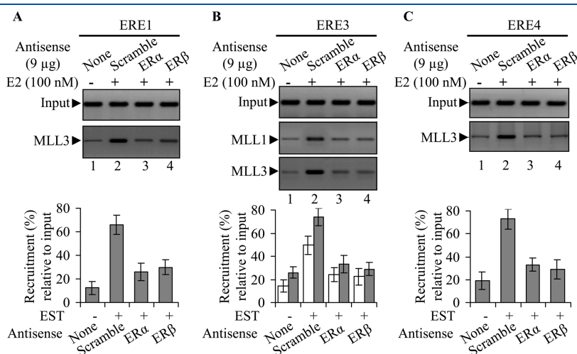
Figure 8. Effects of ER \alpha and ER \beta knockdown on recruitment of MLL1 and MLL3 on ERE1, ERE3, and ERE4 of HOXB9 promoter. JAR cells were transfected with ER \alpha and ER \beta antisenses separately for 48 h followed by exposure to E2 (100 nM for an additional 6 h). Cells were harvested and subjected to ChIP assay using anti-MLL1 and anti-MLL3 antibodies. The immunoprecipitated DNA fragments were PCR-amplified using primer specific to ERE1, ERE3, and ERE4 regions of HOXB9 promoter. Lane 1: control cells (no E2 control). Lanes 2–4 are E2-treated samples. Real-time quantification of recruitment level (% relative to input) is plotted in respective bottom panels. Bars indicate standard errors.
