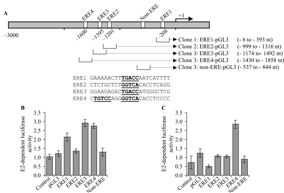
Figure 2. Analysis of HOXB9 promoter EREs and their E2-response using luciferase based reporter assay. (A) HOXB9 promoter (up to -3000 nt) contains three ERE 1/2 sites named as ERE1 to ERE3 and an imperfect full EREs (ERE4). The promoter segments containing these ERE 1/2 sites along with \sim 150 nt on both sides were cloned into luciferase based reporter construct pGL3 and used for transfection. (B) E2-response of HOXB9 promoter EREs in JAR cells. The ERE containing pGL3 constructs were transfected into JAR cells for 24 h. Control cells were treated with either none (no construct transfected, control lane) or empty pGL3 vector or non-ERE-pGL3 (non-ERE). Both control and plasmid transfected cells were then treated with 100 nM E2 for 6 h and subjected to luciferase assay by using ONE-Glo luciferase assay system. The ratio of E2-induced luciferase activities over corresponding E2-untreated samples was plotted. The experiment with four replicate treatments was repeated at least twice. Bars indicate standard errors. (C) E2-response of HOXB9 promoter EREs in MCF7 cells. Experiments were performed in MCF7 cells in the same way as described in (B).
